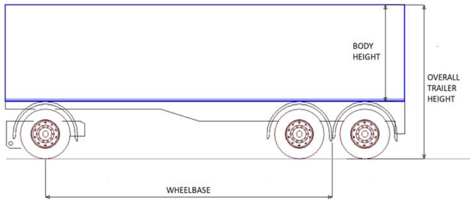
Figure 1 - 3 Axle Dog Measurement Example
