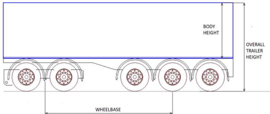
Figure 3 - 5 Axle Dog Measurement Example
